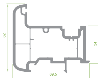
PRP.7600 Mullion Rebate Profile
