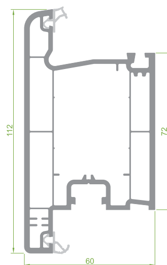
PRP.6500 Outer Doorsash Profile
