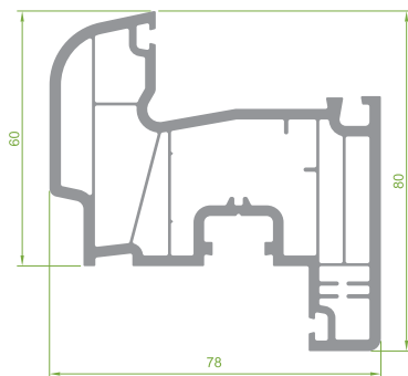
PRP.7500 Super Sash Profile
