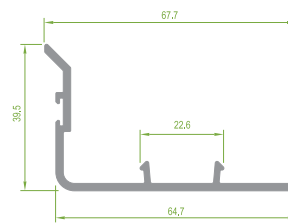
PRP.5350 Wide Sliding System Rear Closing Profile
