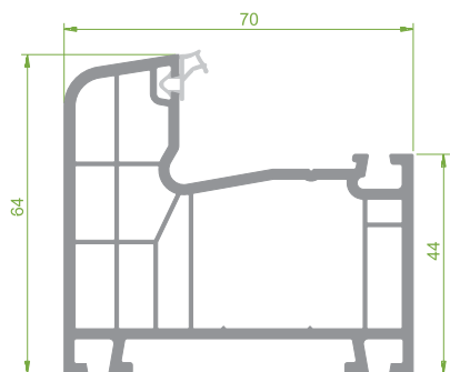
PRP.7140 Frame Profile
