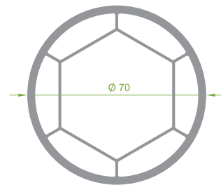
PRP.8110 Pipe Profile
