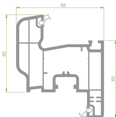
PRP.7540 Sash Profile
