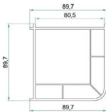
TML.8120 90° Corner Connection Profile
