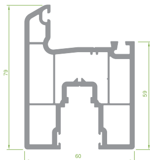
PRP.5250 Wide Sliding Sash Profile
