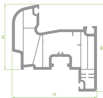
PRP.7500 Super Sash Profile
