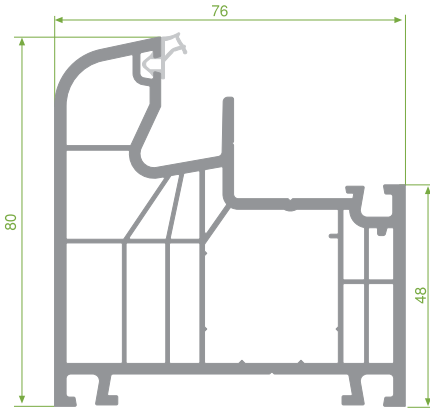
PRP.7170 Frame Profile
