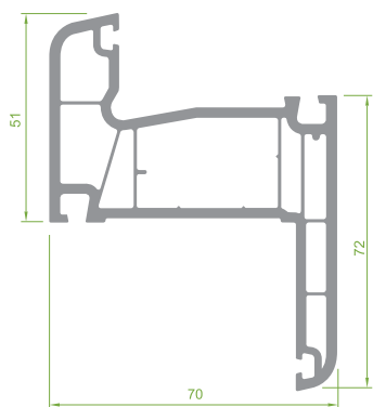
PRP.7700 Frame Profile With Border
