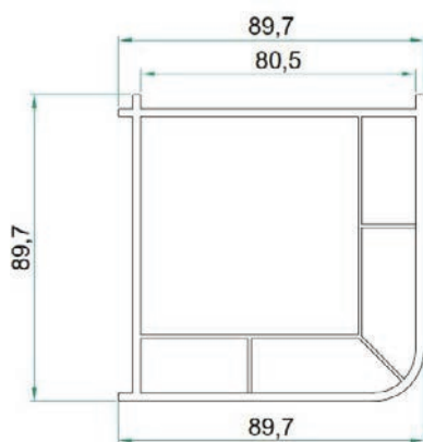
TML.8120 90° Corner Connection Profile
