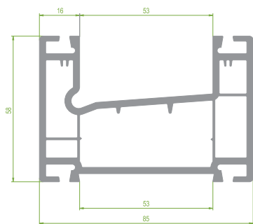
PRP.5150 Wide Sliding Frame Profile
