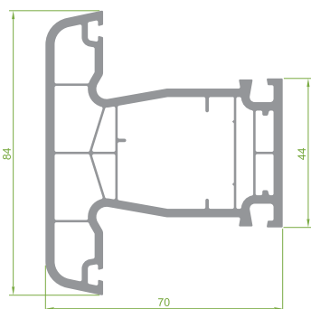
PRP.7300 Transom Profile
