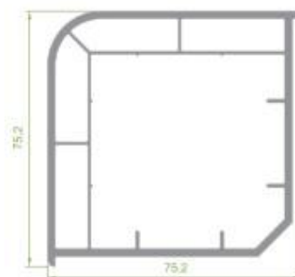
PRP.6910 90° Corner Turning Profile
