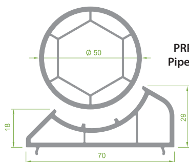
PRP.7900 Angled Corner Turning Adaptor Profile
