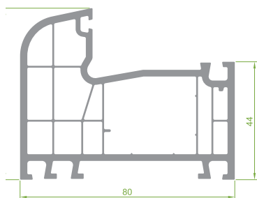
PRP.8100 Frame Profile
