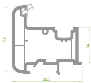
PRP.6600 Mullion Rebate Profile
