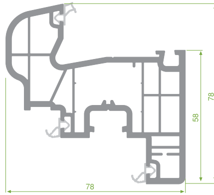
PRP.7570 Super Sash Profile
