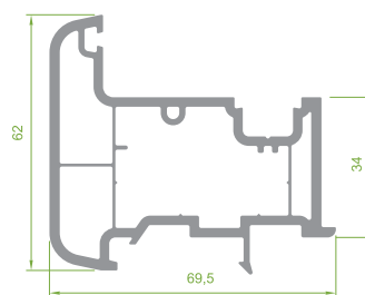
PRP.7600 Mullion Rebate Profile
