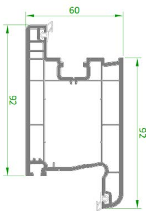
PRP.6420 Wide Door Sash Profile "92 mm"
