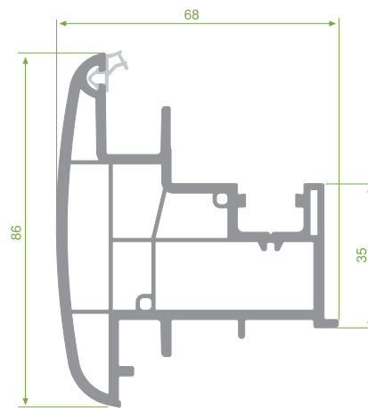
PRP.7640 Mullion Rebate Profile
