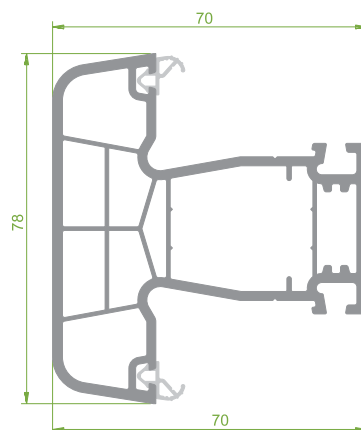
PRP.7340 Transom Profile
