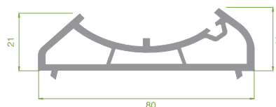
TML.8100 Angled corner Connection Profile
